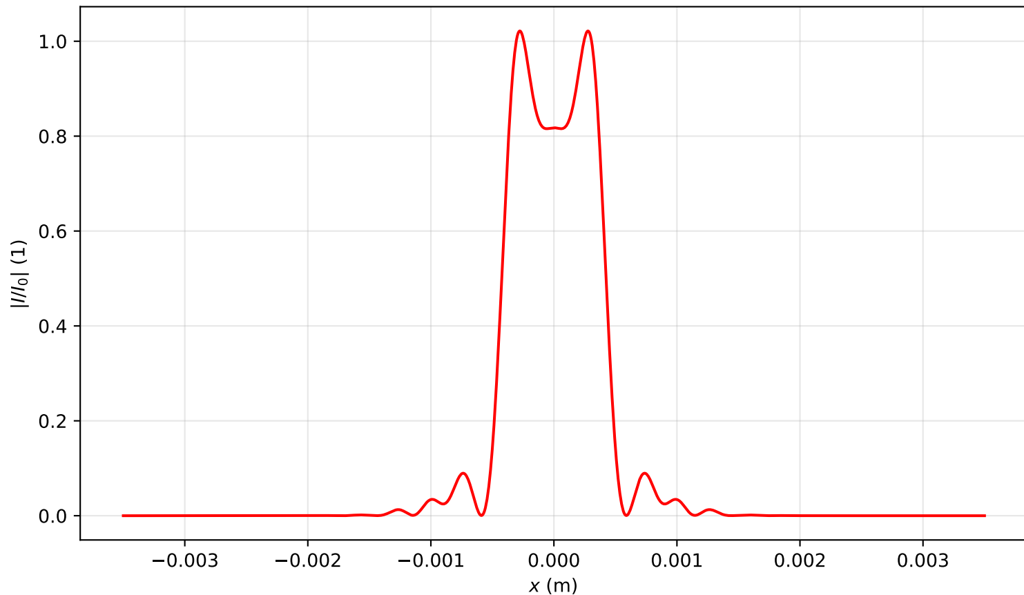
Intensity profile I(x, y = 0, z = 1.194)/I_0 , P_{in}=3.0P_{cr} , artificial time
